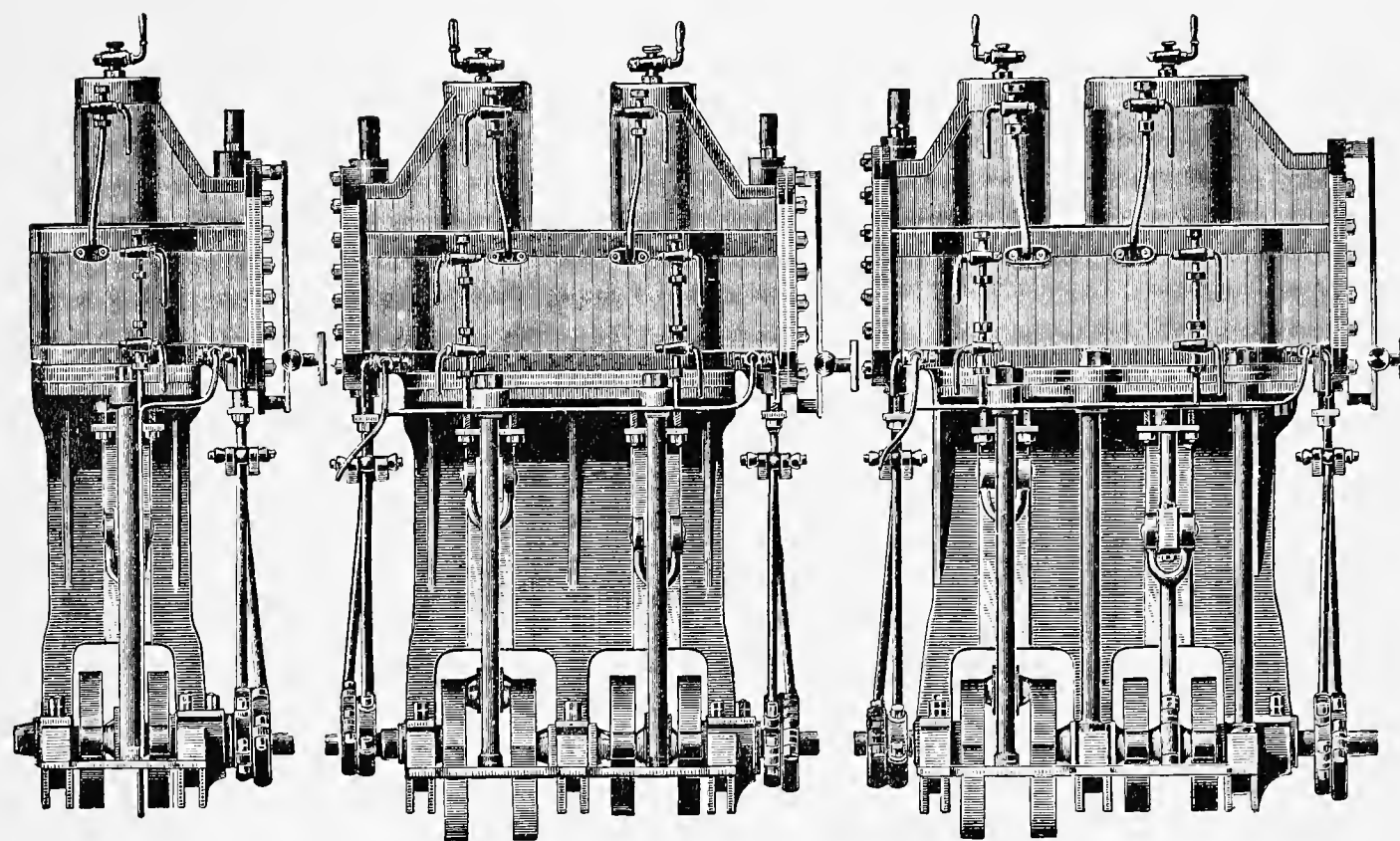
SINGLE COMPOUND.
